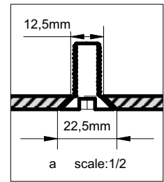
Flat head socket cap screw DIN7991 M10X25
