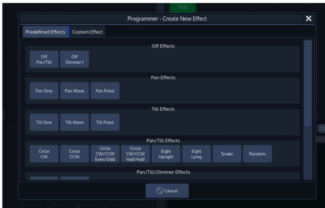
Fig. 121: Predefined Effects
