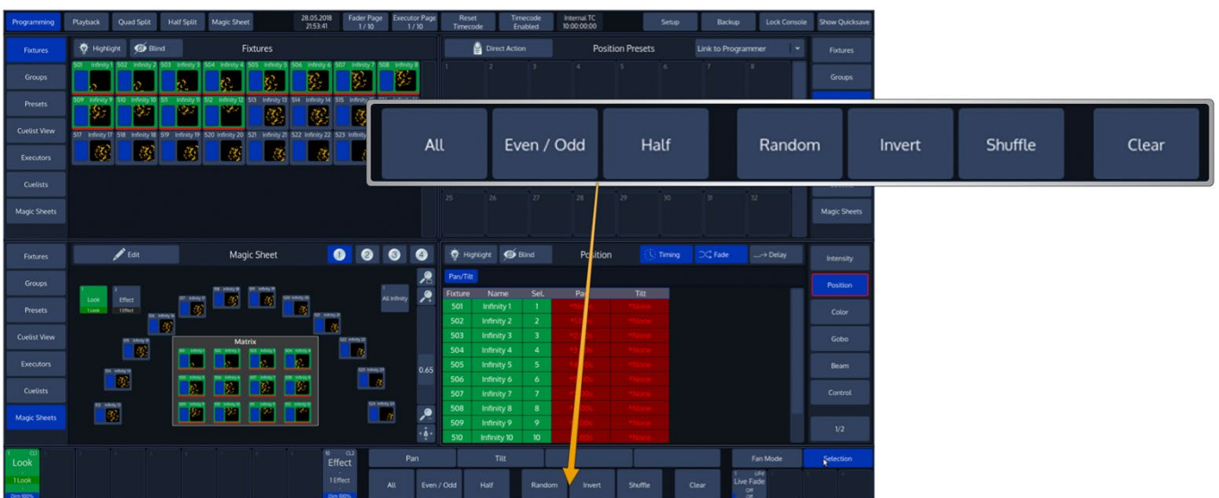
Fig. 85: Selection Toolbar
