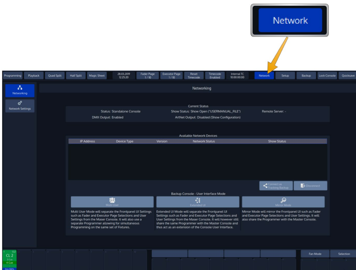
Fig. 198: Network Screen
