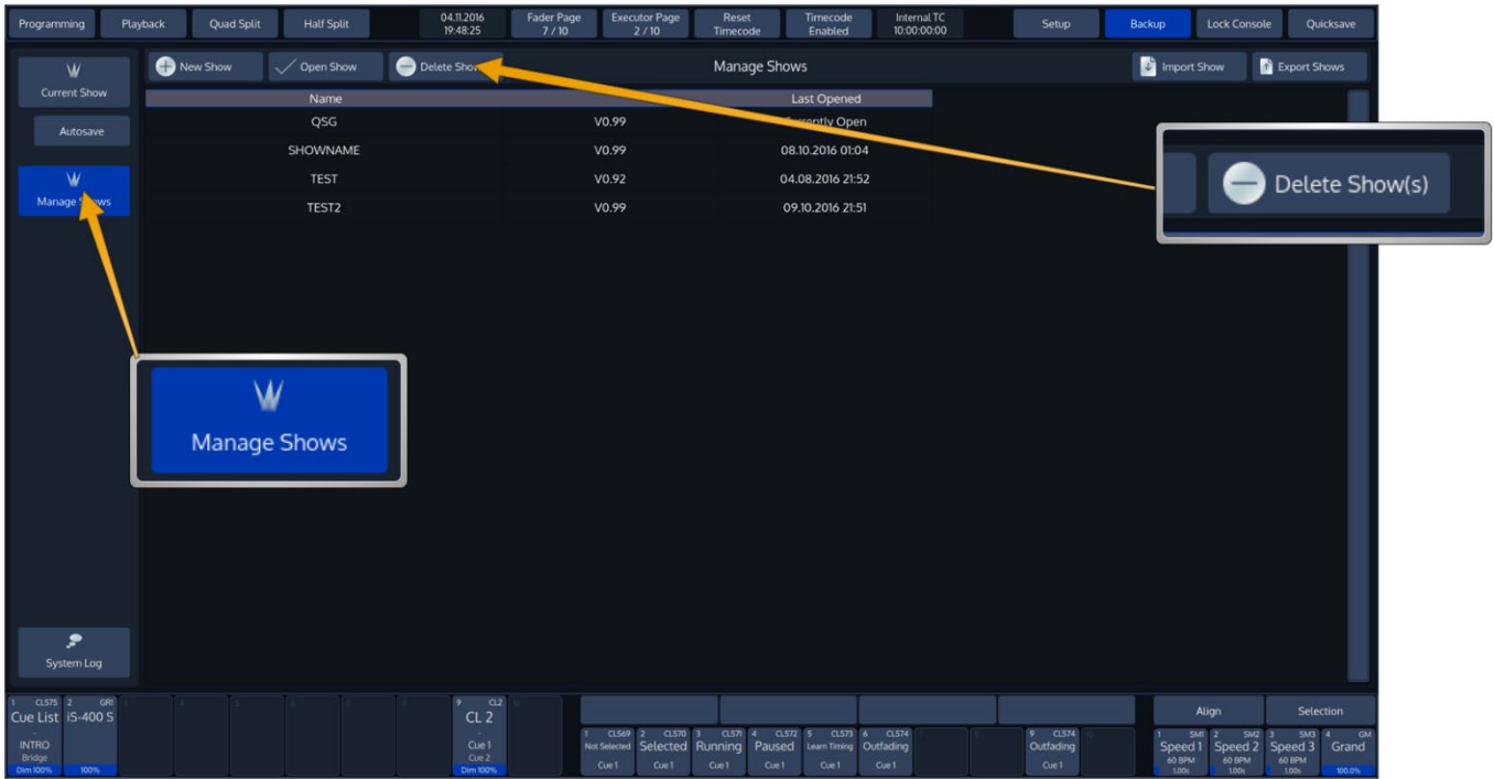
Fig. 44: Delete Shows
