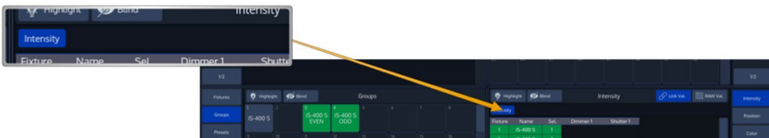
Fig. 94: Attribute Selection
