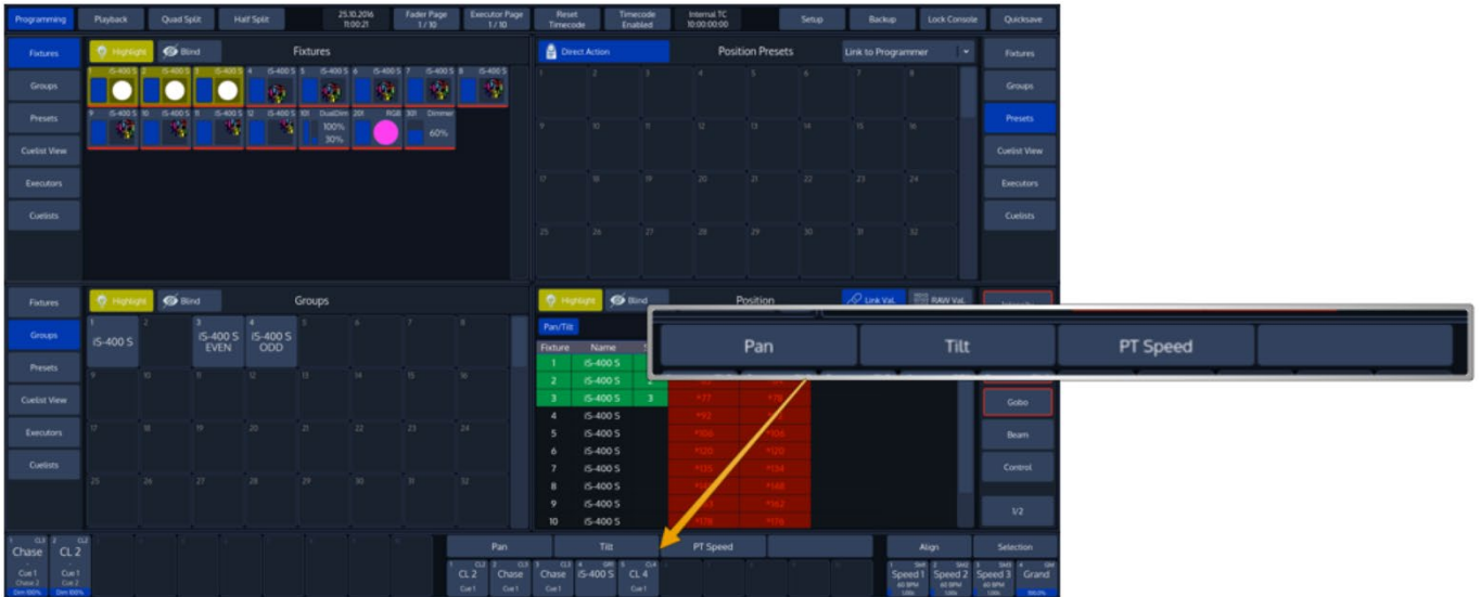
Fig. 20: Encoder Labels
