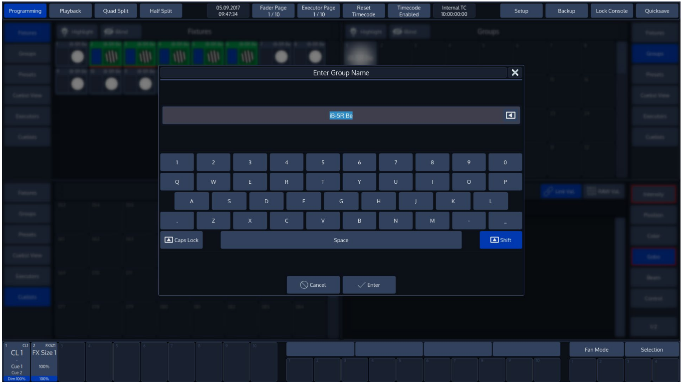
Fig. 34: Keyboard Dialog
