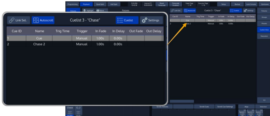
Fig. 149: Cuelist View
