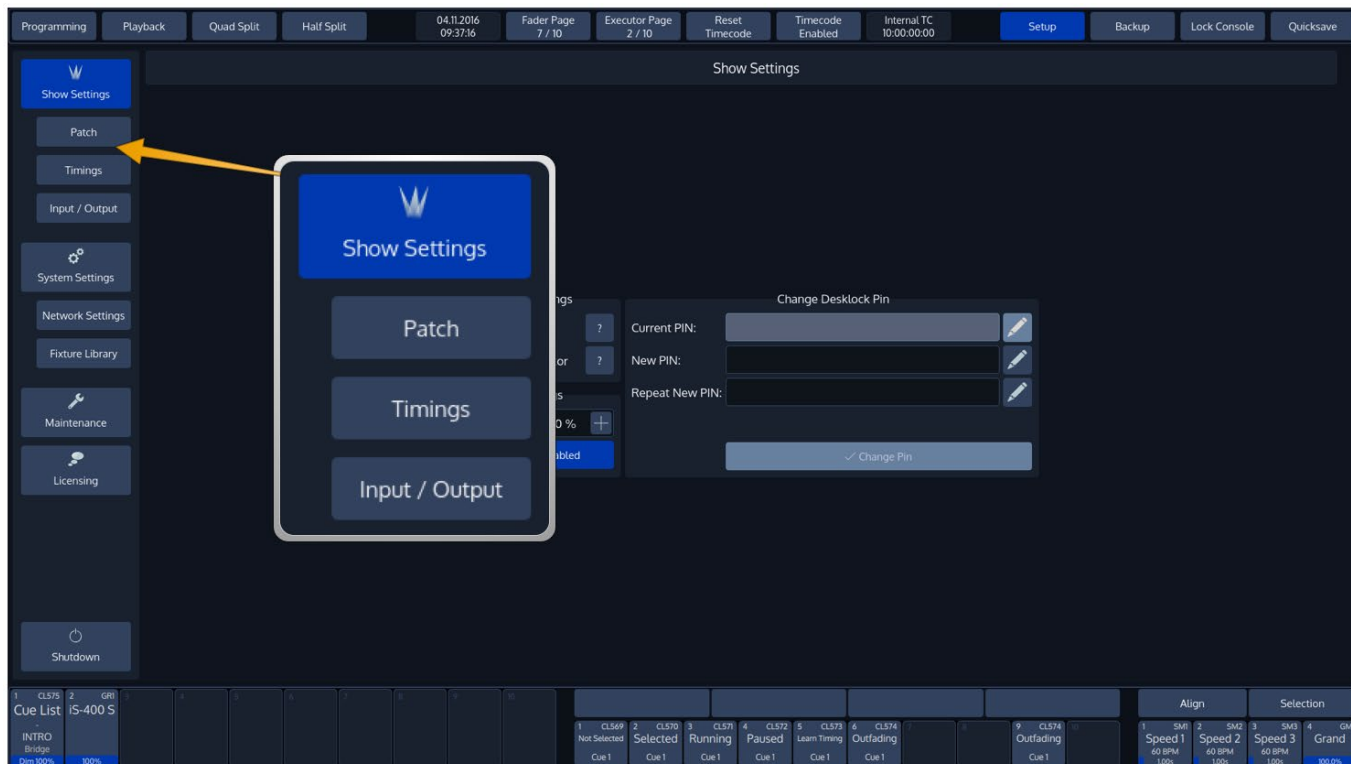
Fig. 45: Show Settings
