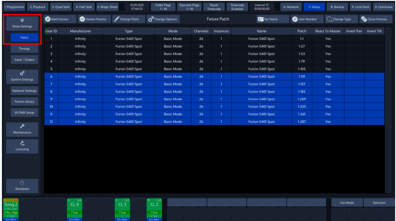
Fig. 50: Patch Screen
