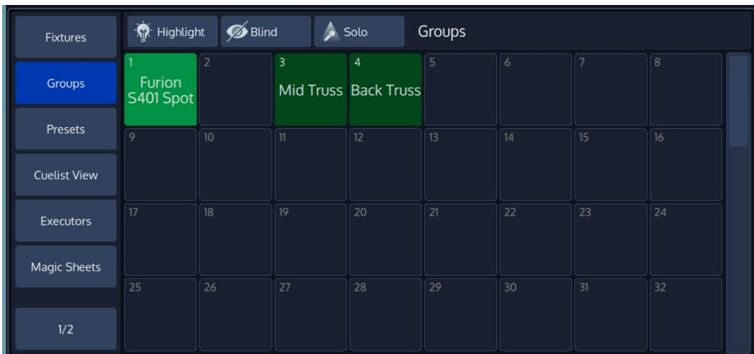
Fig. 88: Group Pool
