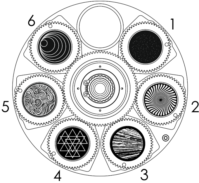
Gobo wheel 1
