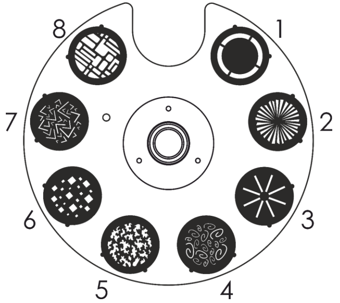
Gobo wheel 2
