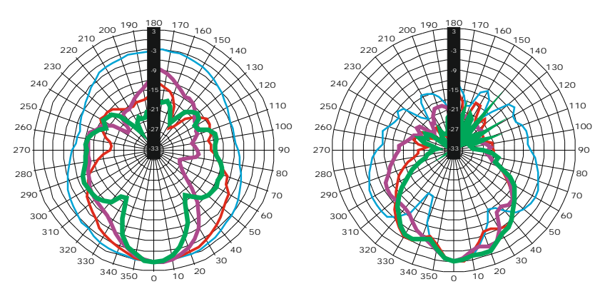
VERTICAL POLAR DIAGRAM Legend: 250 (blue), 500 (red), 800 (magenta), 1000 (green), 1400 (cyan), 2000 (orange), 2500 (purple), 3150 (dark green)
