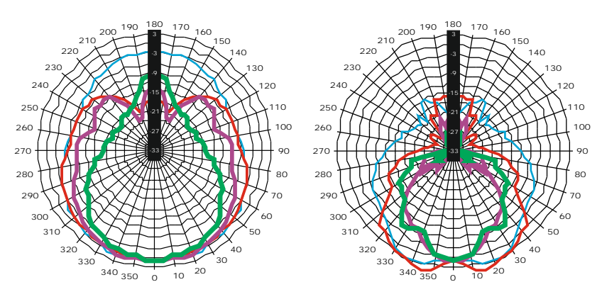
HORIZONTAL POLAR DIAGRAM Legend: 250 (blue), 500 (red), 1000 (magenta), 2000 (green), 4000 (cyan), 8000 (orange), 12500 (purple), 16000 (dark green)
