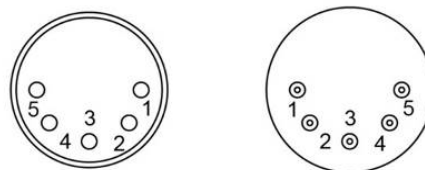
5 Pin XLR
