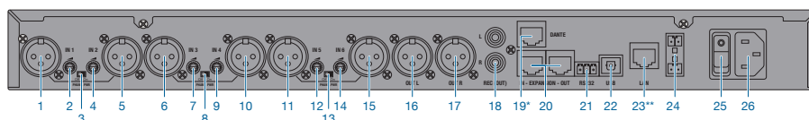
Figure 2: Rear of the DMM8 U (UL, ULD)
