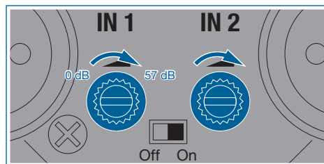
Figure 4: Gain controller
