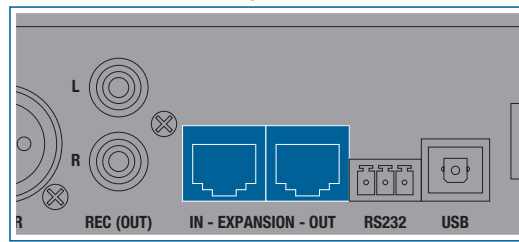
Figure 10: Expansion
