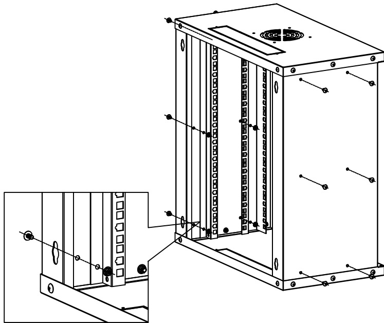
A:M5x10 Phillips flat head screws 12PCS B:M5 Hexagonal flange nuts 12PCS
